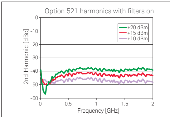
Harmonics (measured)
